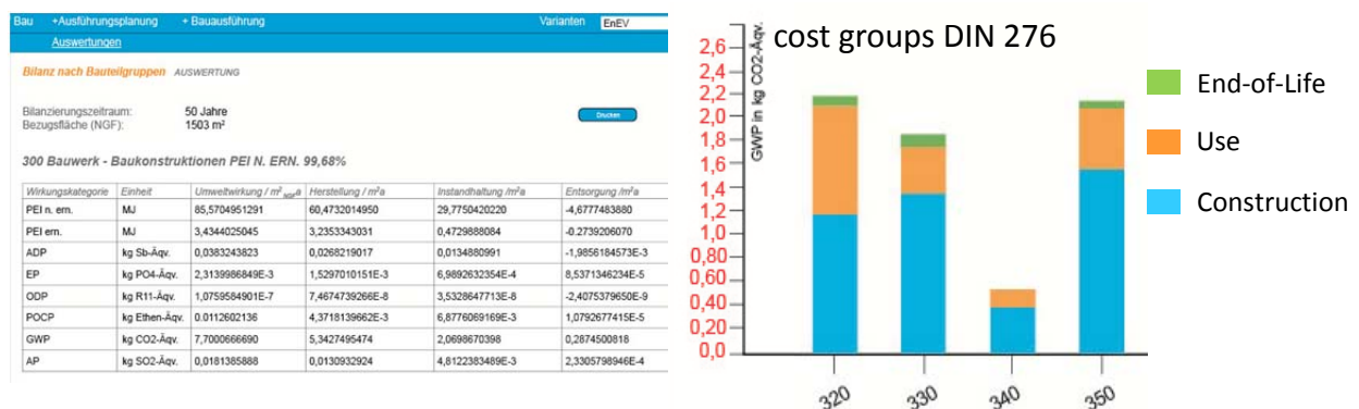
Figure 6: eLCA - Total score result and separation of results to cost groups and life cycle stages (left: table of results for environmental indicators; right: results of GWP in cost groups and life cycle stages)
